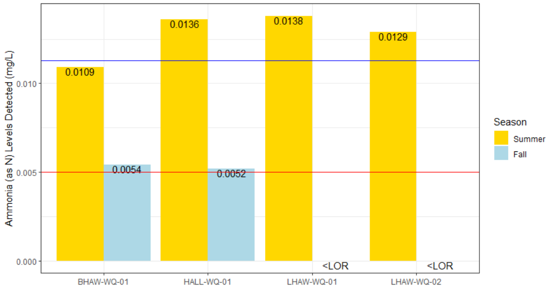
Figure 3: HHLPOA Lakes ammonia results, 2022. The red trendline represents the limit of reporting for ALS laboratories while the blue trendline represents the level of ammonia concentrations detected at the reference site on Stocking Lake.
