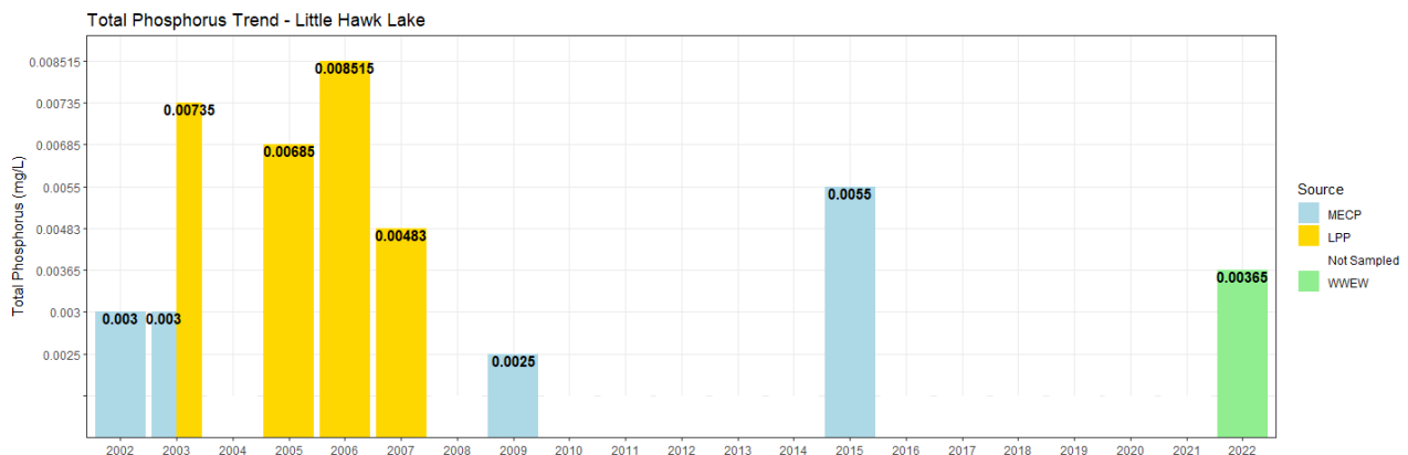
Figure 6: Total phosphorus trend in Little Hawk Lake (45.1450421, -78.7202599)
