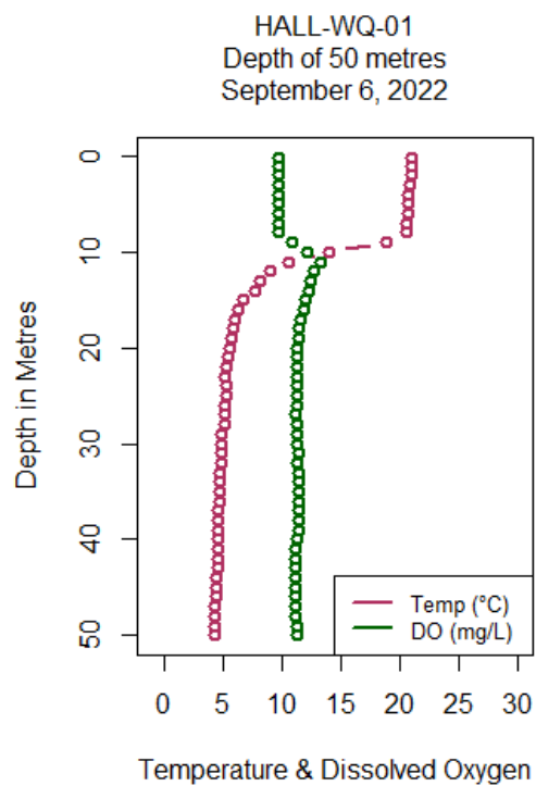
Figure 5 (a-h): Temperature and dissolved oxygen profiles for all sites, 2022
